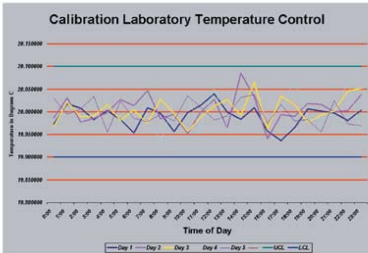
Computer controlled Lab environment allows for constant temperature monitoring.
